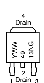
1 Drain 2 Gate 3 Source 4 Drain
