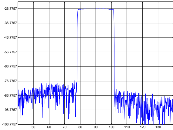
Group Delay Variation( f_0 \pm 11.5\text{Hz} )
