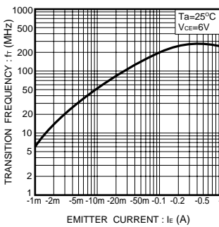
Fig.8 Gain bandwidth product vs. emitter current
