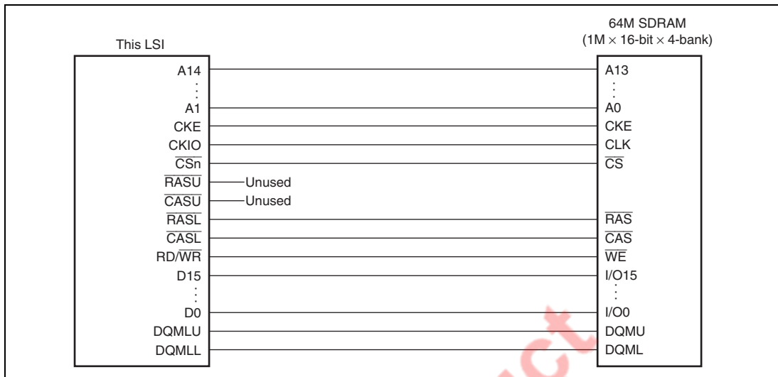
Figure 12.16 Example of 16-Bit Data Width SDRAM Connection ( \overline{\text{RASU}} and \overline{\text{CASU}} are Not Used)
