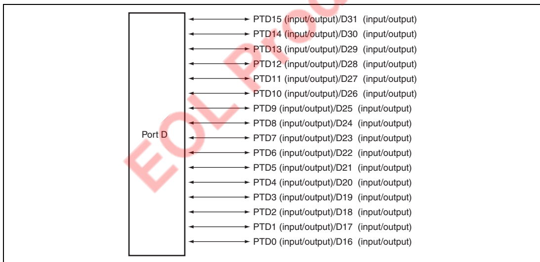
Figure 23.4 Port D
