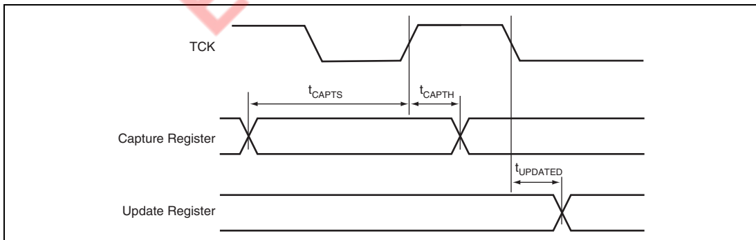
Figure 25.54 Boundary-Scan Input/Output Timing
