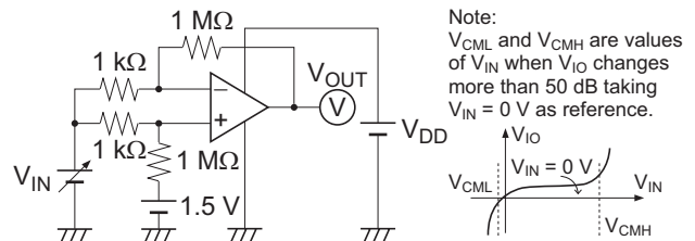
8. Common Mode Input Voltage Range, V_{CM}
