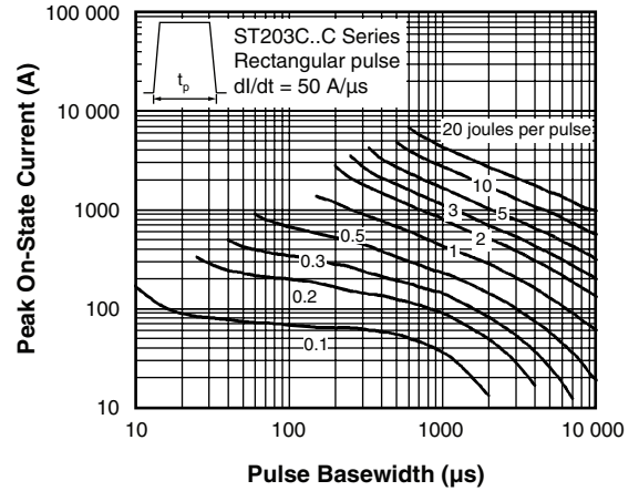
Fig. 16 - Maximum On-State Energy Power Loss Characteristics
