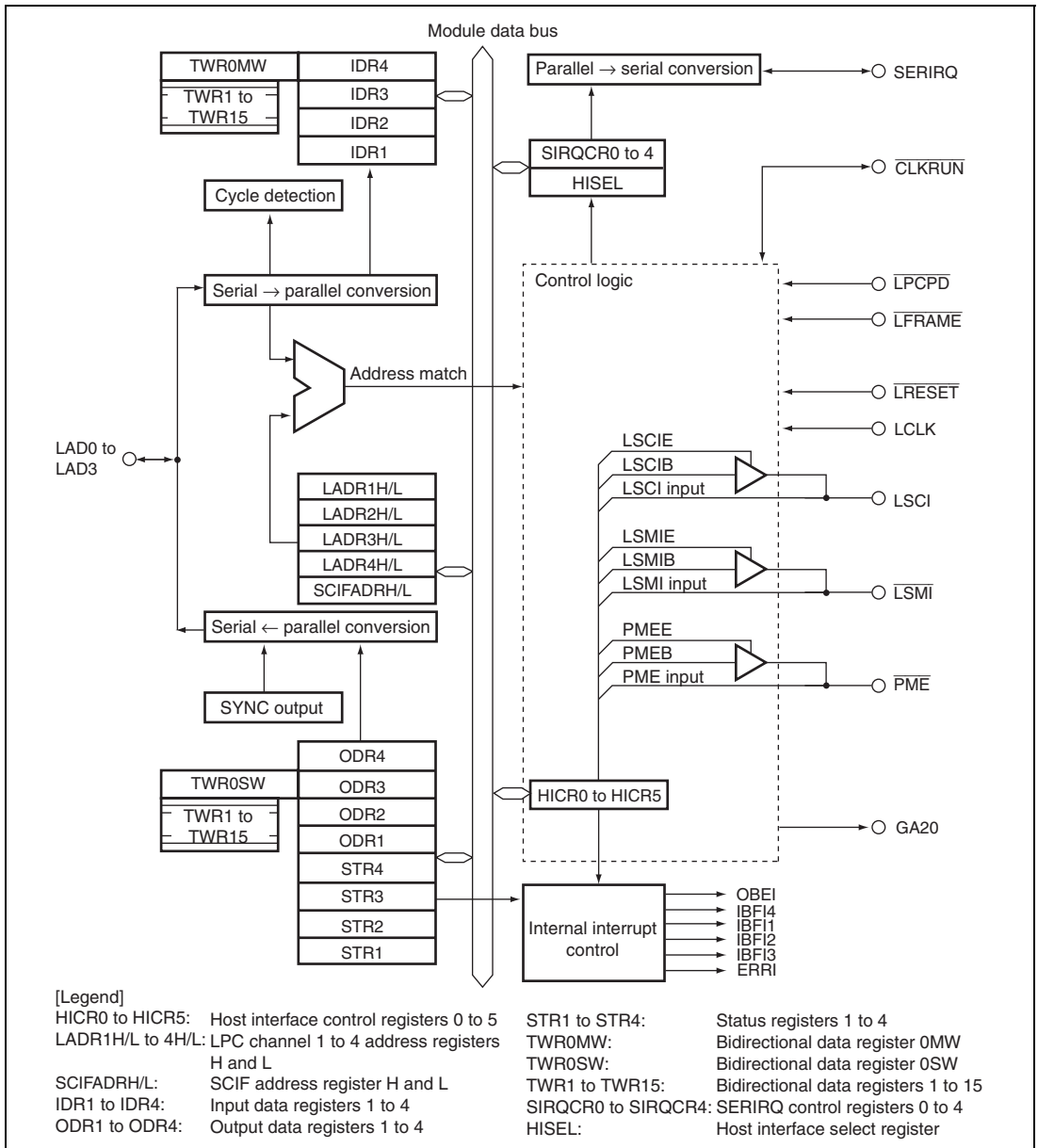
Figure 19.1 Block Diagram of LPC
