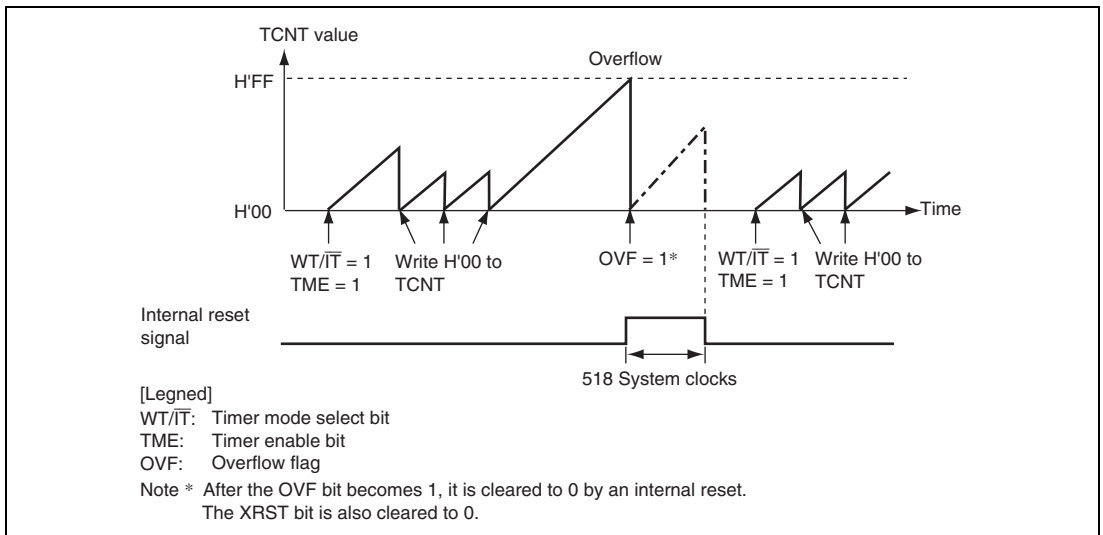
Figure 14.2 Watchdog Timer Mode ( \overline{RST}/\overline{NMI} = 1 ) Operation
