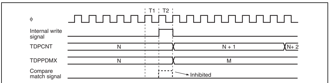
Figure 12.14 Conflict between TDPPDMX Write and Compare Match
