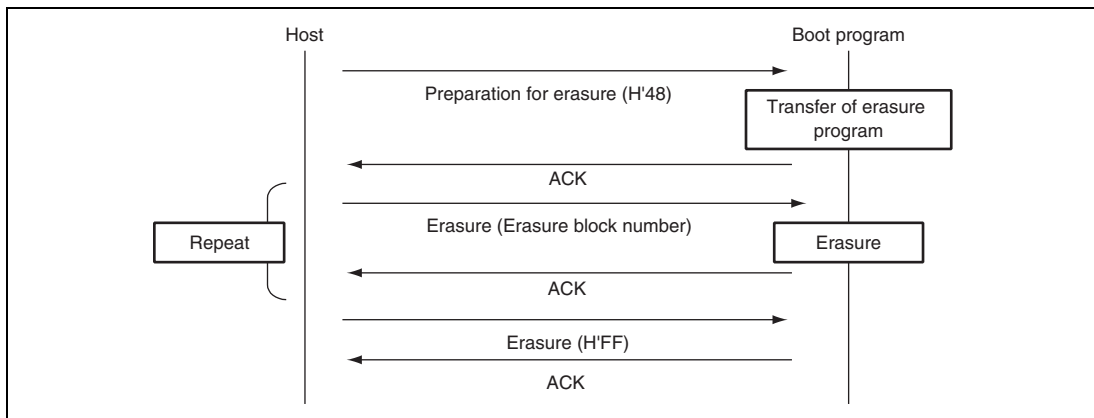
Figure 22.23 Erasure Sequence
