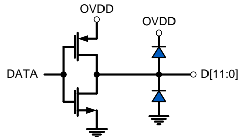
FIGURE 48. CMOS OUTPUTS
