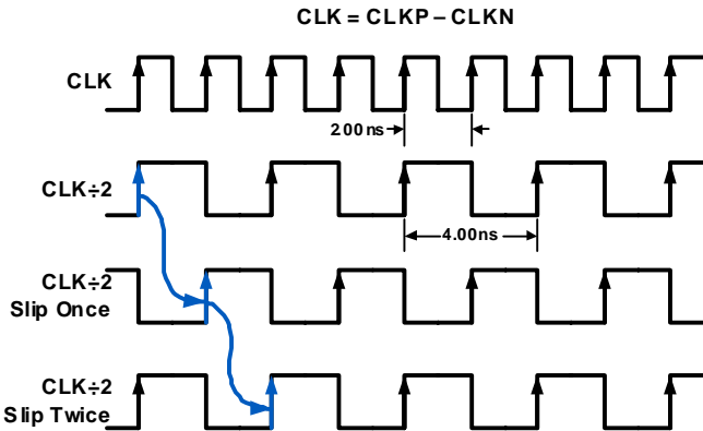
FIGURE 40. PHASE SLIP: CLK÷2 MODE, f CLOCK = 500MHZ
