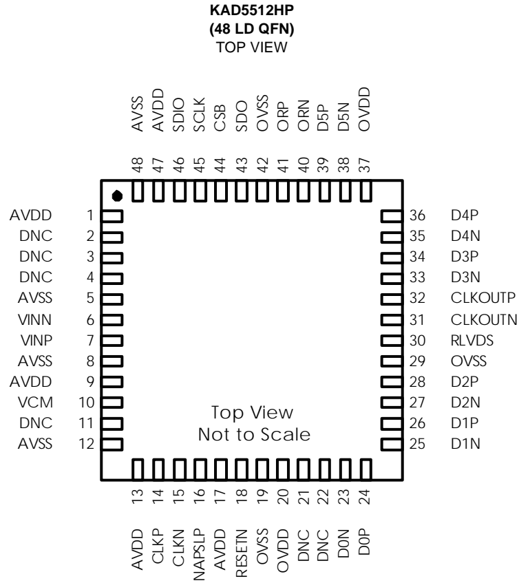
FIGURE 4. 48QFN PIN CONFIGURATION
