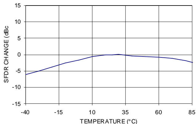
FIGURE 26. SFDR PERFORMANCE vs TEMPERATURE AFTER +25°C CALIBRATION
