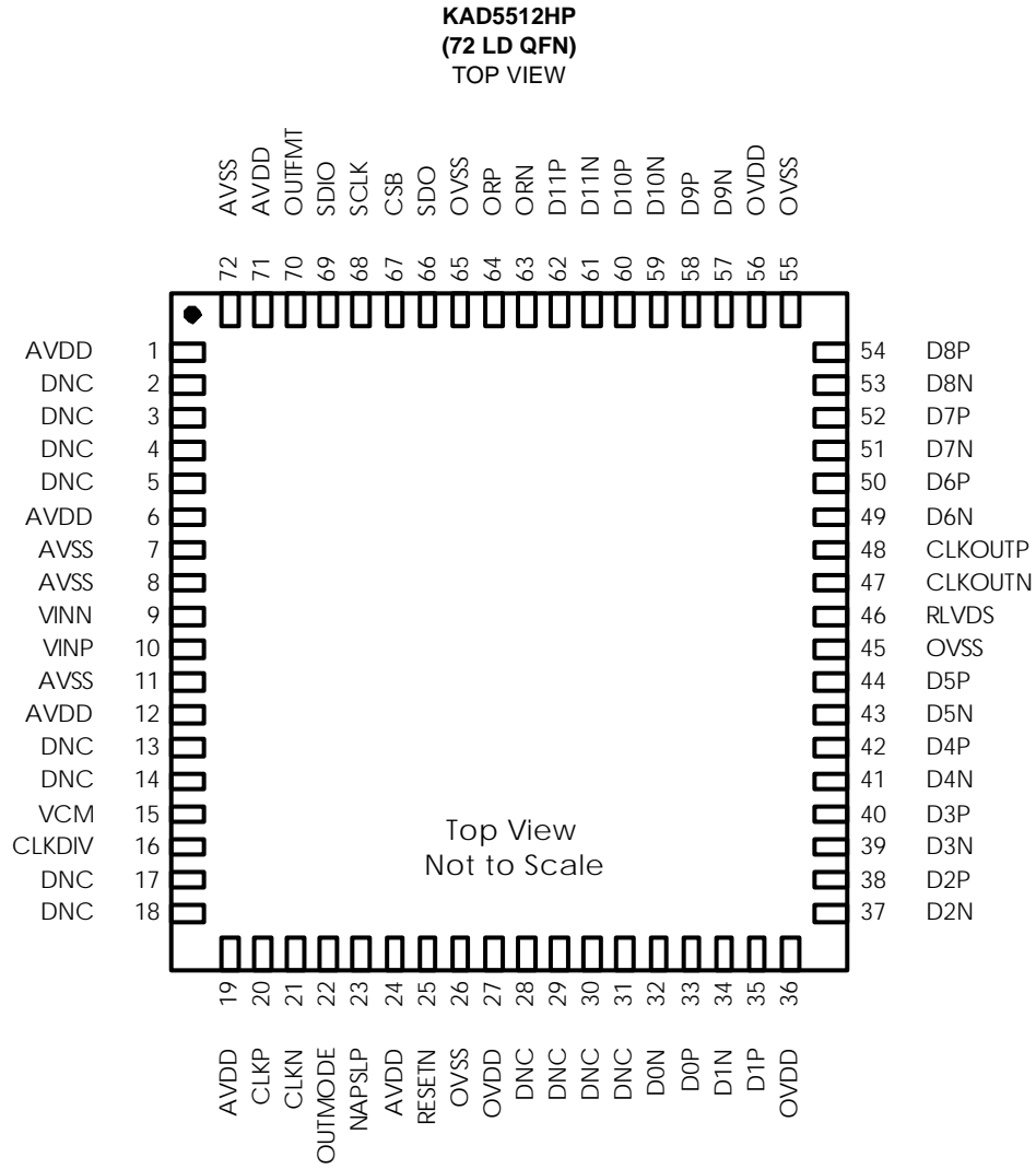
FIGURE 3. 72QFN PIN CONFIGURATION
