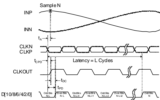
FIGURE 2A. DDR
