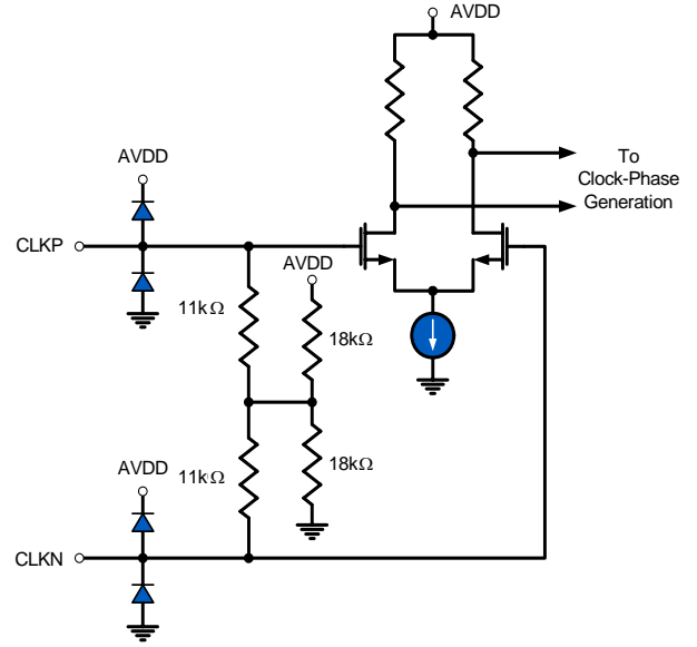
FIGURE 44. CLOCK INPUTS
