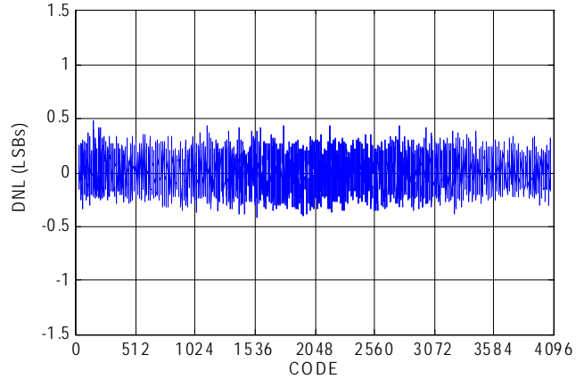
FIGURE 12. DIFFERENTIAL NONLINEARITY
