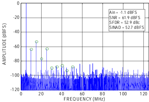
FIGURE 20. SINGLE-TONE SPECTRUM @ 995MHz
