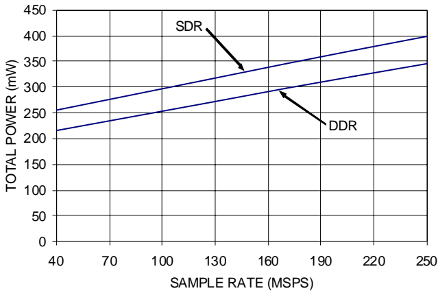
FIGURE 11. POWER vs fSAMPLE IN 3mA LVDS MODE
