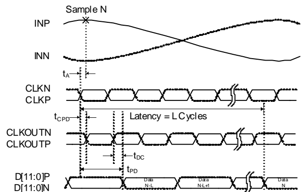
FIGURE 1B. SDR
