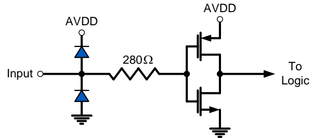
FIGURE 46. DIGITAL INPUTS
