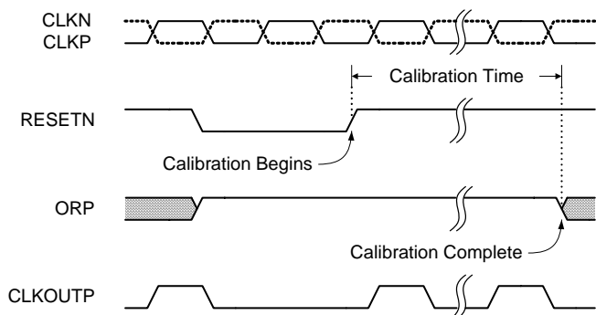
FIGURE 24. CALIBRATION TIMING
