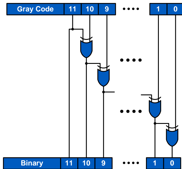
FIGURE 34. GRAY CODE TO BINARY CONVERSION
