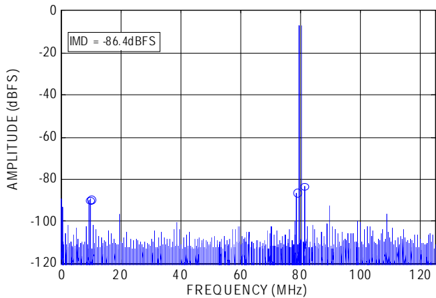
FIGURE 22. TWO-TONE SPECTRUM @ 170MHz
