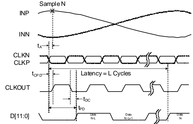
FIGURE 2B. SDR
