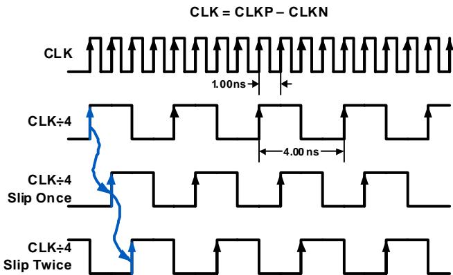
FIGURE 41. PHASE SLIP: CLK÷4 MODE, f CLOCK = 1000MHZ
