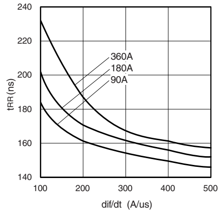
Fig. 4 - Typical Reverse Recovery Time vs. di_F/dt T_J = 125^\circ\text{C} (Per Leg)
