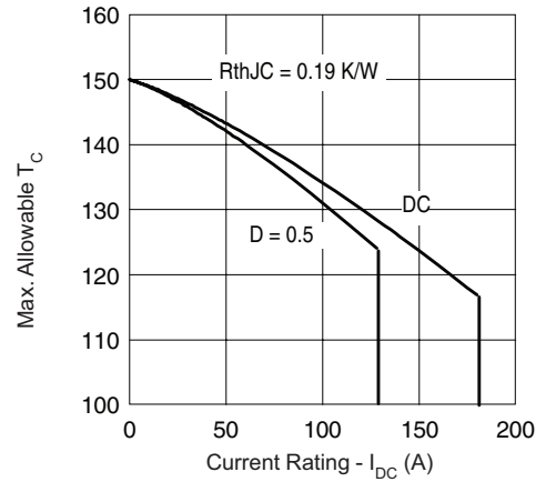
Fig. 3 - Maximum Current Rating Capability (Per Leg)
