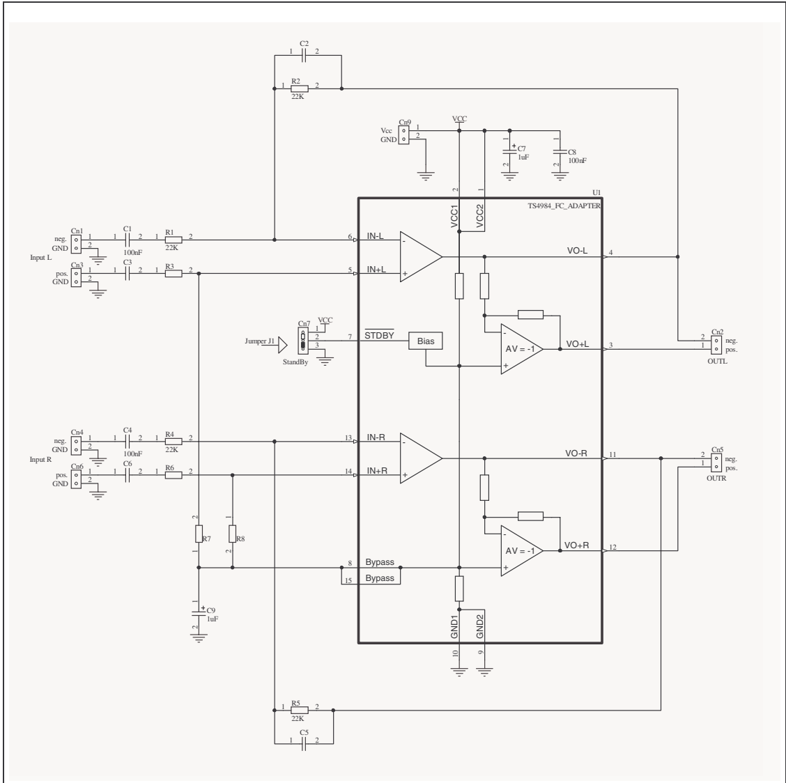
Figure 71. Demoboard schematic
