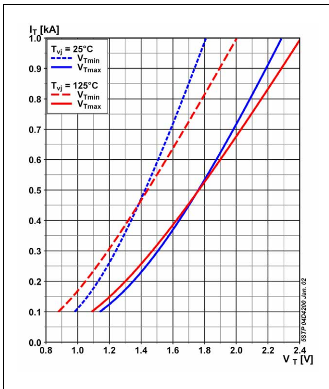
Fig. 2 On-state characteristics.
