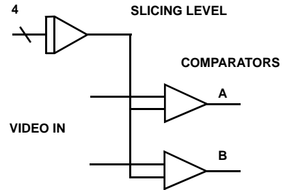
FIGURE 14. DELAY DETECTOR
