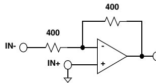
FIGURE 2. A_V = -1
