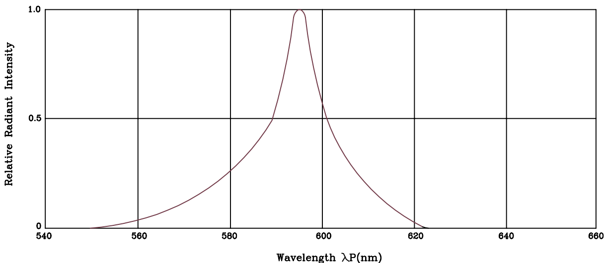
SPECTRAL DISTRIBUTION
