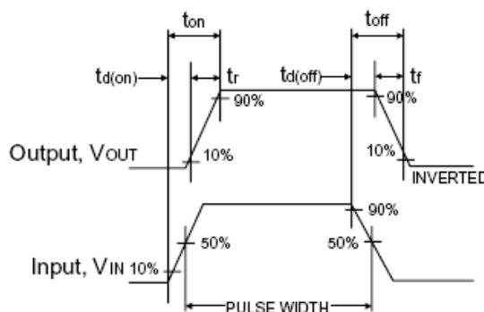
Switchin Waveforms
