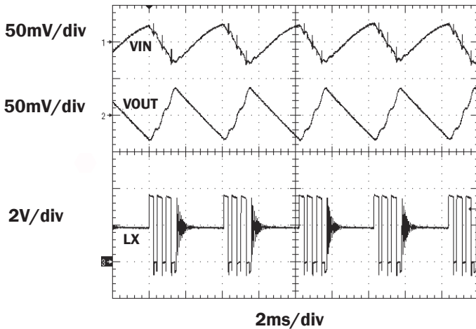
PSAVE @ 50mA Load
