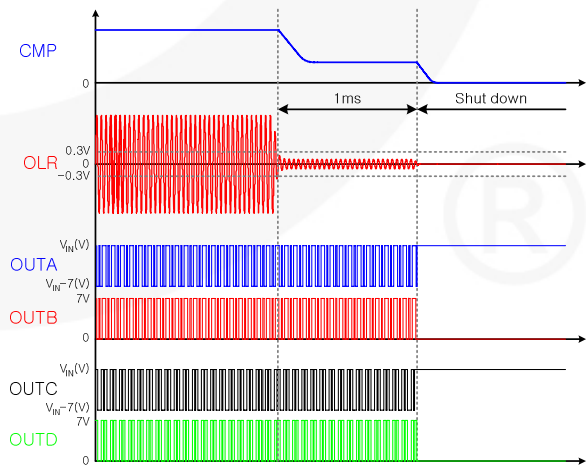
Figure 53. Short-Lamp Protection
