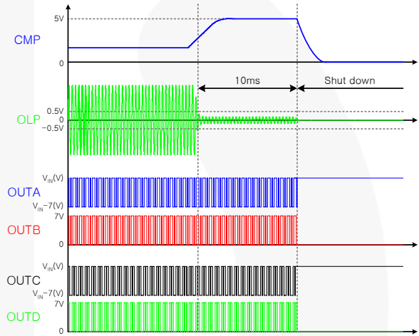
Figure 52. Open-Lamp Protection in Normal Mode
