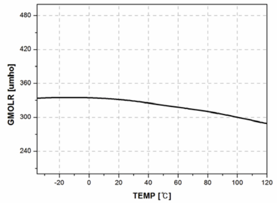
Figure 30. OLR Error Amp. GM vs. Temp.
