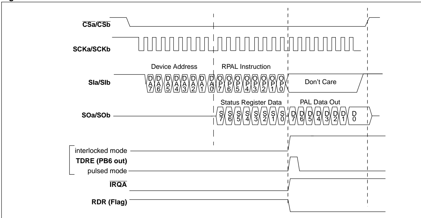
Figure 20. Bi-directional Mode - SPI Read
