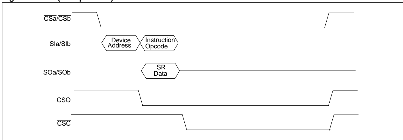
Figure 2. NOP (No Operation)
