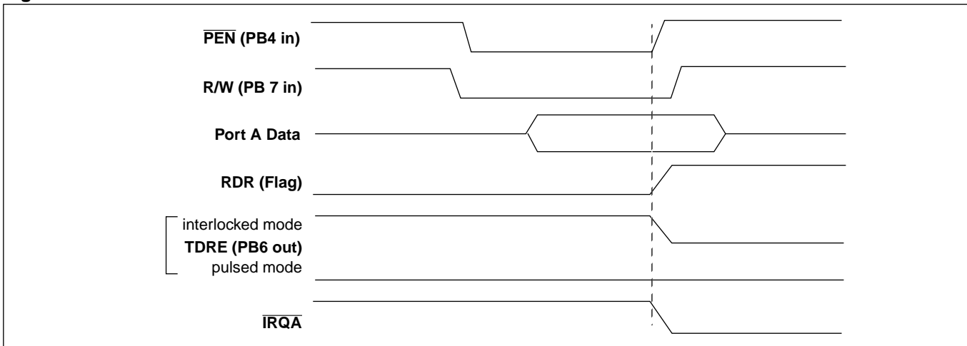
Figure 19. Bi-directional Mode - Parallel Write
