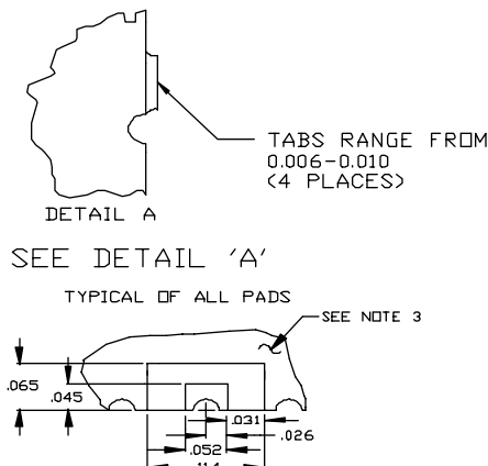
PHYSICAL DIMENSIONS
