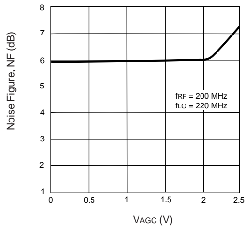
NOISE FIGURE vs. V_{AGC}
