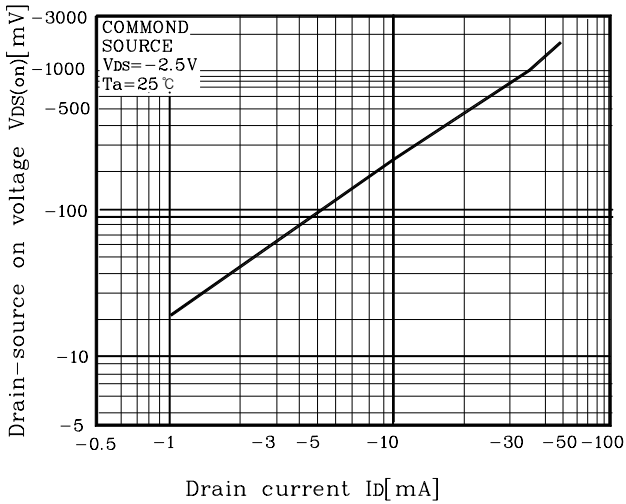
Fig7 VDS(on) - Id
