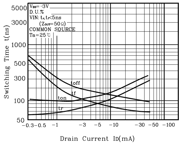
Fig8 t - Id
