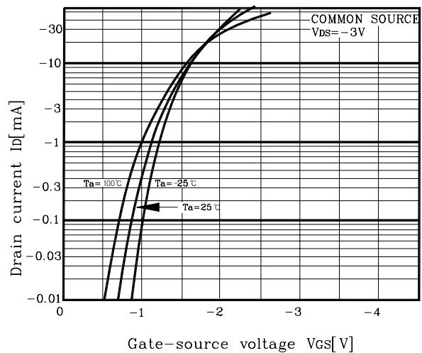
Fig4 I D - V GS
