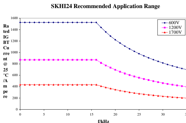
Fig. 5 shows the recommended maximum switching frequencies for SEMIKRON Semitrans IGBT modules.
