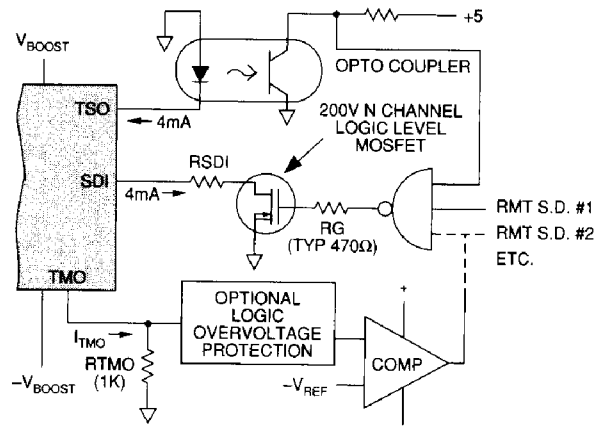
FIGURE 9. EXTERNALLY CONTROLLED THERMAL PROTECTION
