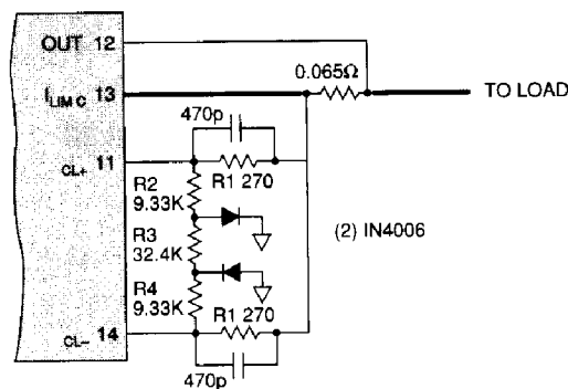
FIGURE 4. FOLDOVER CURRENT LIMIT
