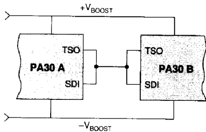
FIGURE 7. SIMPLE TSO/SDI LOOP
