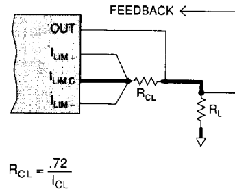
FIGURE 1. I_{LIMIT} WHERE I_{CL+} = I_{CL-}
