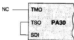
FIGURE 8. SIMPLE TSO/SDI LOOP
