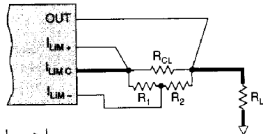
FIGURE 3. I_{LIMIT} WHERE I_{CL+} \neq I_{CL-} When doing unbalanced current limit, watch for voltage drop on R_{CL} and dissipation in R_{CL} .
