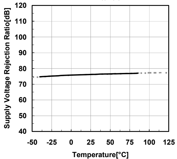
Supply Voltage Rejection Ratio vs. Temperature V+/V- = \pm 1.1V\ to\ \pm 3.5V
