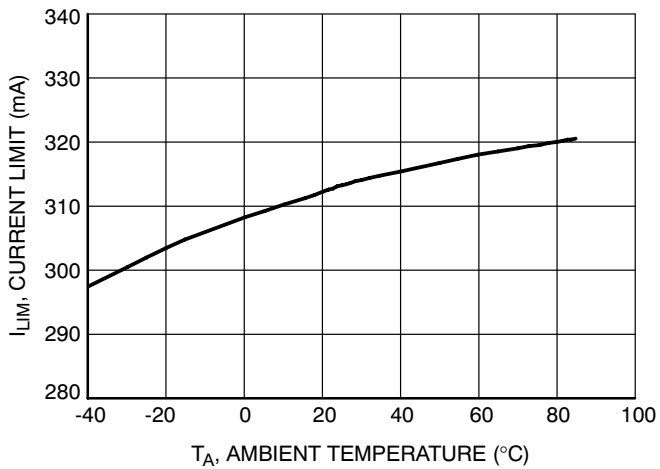
Figure 11. Current Limit vs. Temperature
