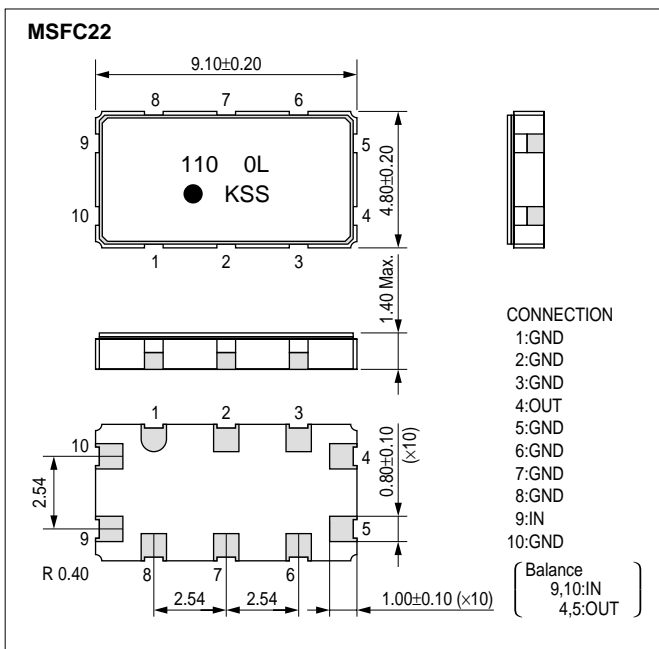
Dimensions(mm)
