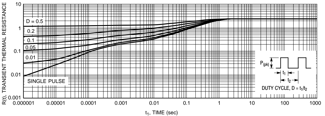
Figure 9. Thermal Response Junction-to-Case for MBRF30H60CTG
