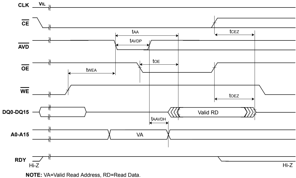
Figure 31. Asynchronous Read Mode( \overline{AVD} toggling)
