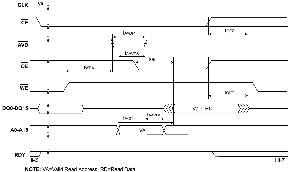
Figure 32. Asynchronous Read Mode( \overline{AVD} toggling)
