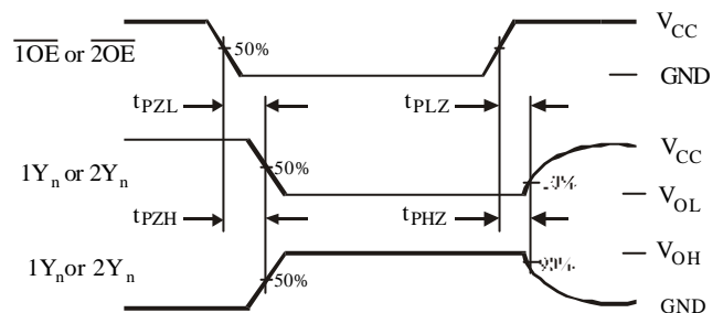
Figure 2. Switching Waveforms
