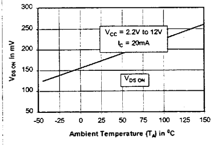
Typical Saturation Voltage vs Temperature
