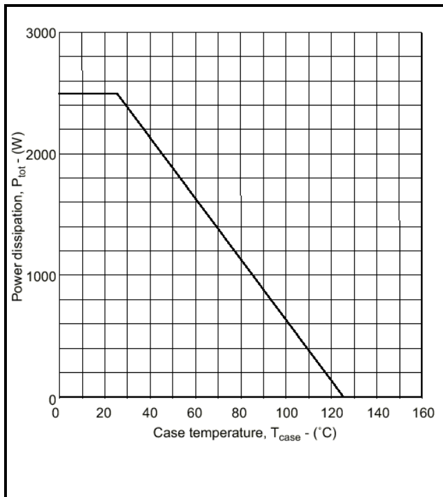
Fig.5 Power dissipation
