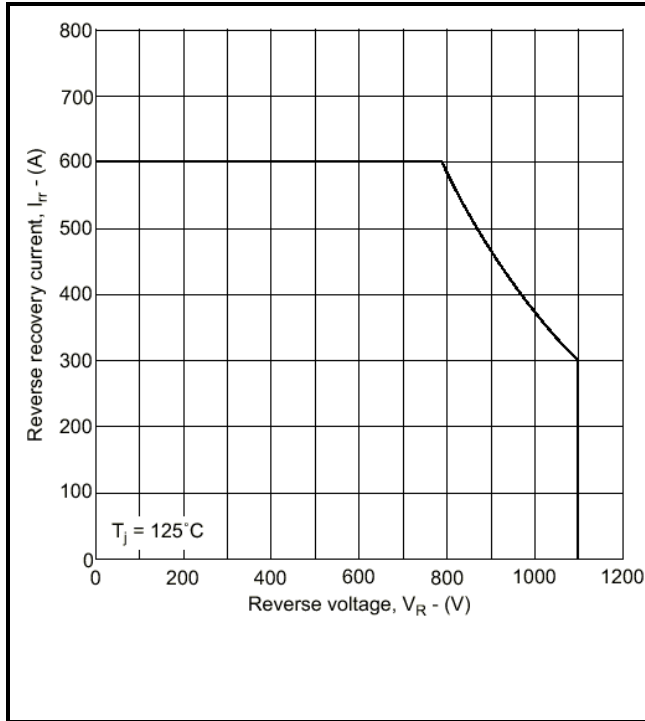
Fig.7 RBSOA
