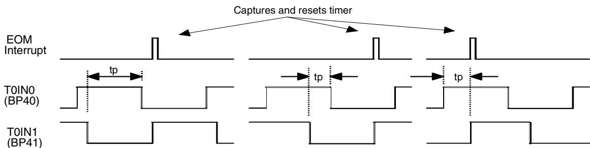
Figure 3-22. Phase Measurement
