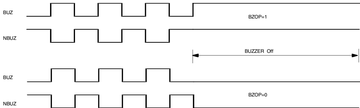
Figure 3-28. Buzzer Waveform
