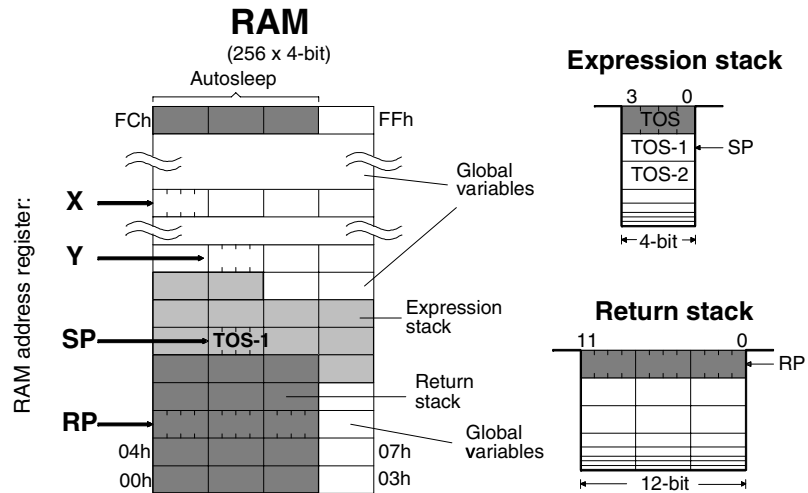
Figure 2-3. RAM Map
