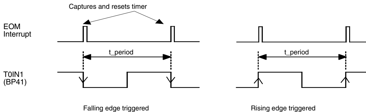
Figure 3-20. Period Measurement
