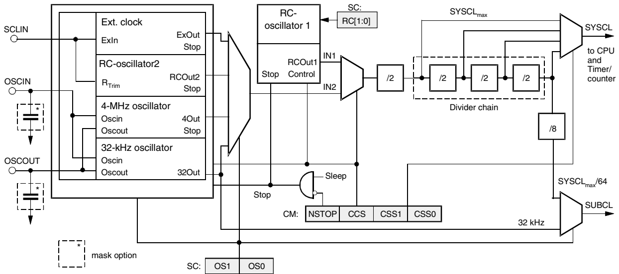
Figure 2-8. Clock Module
