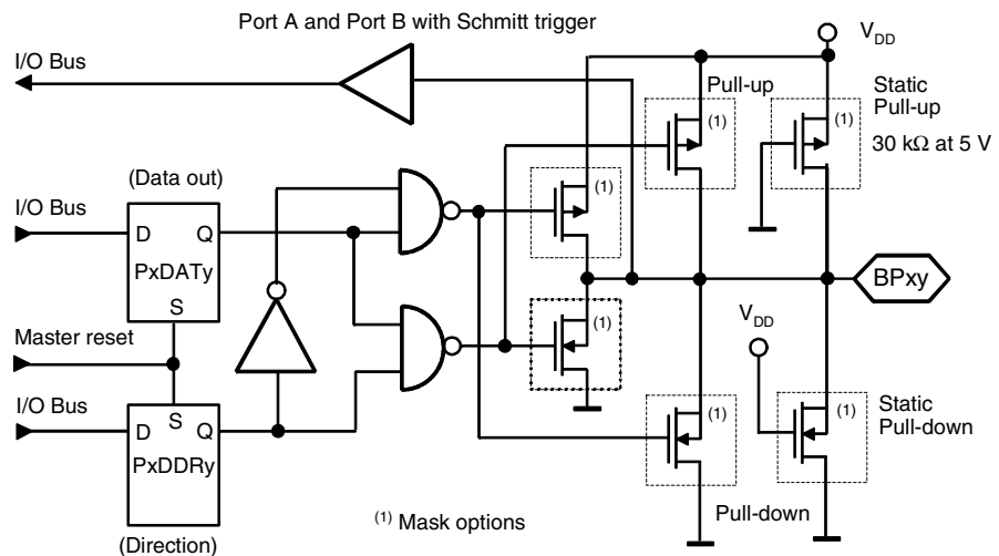
Figure 3-3. Bi-directional Ports 5, 7, A, B and C
