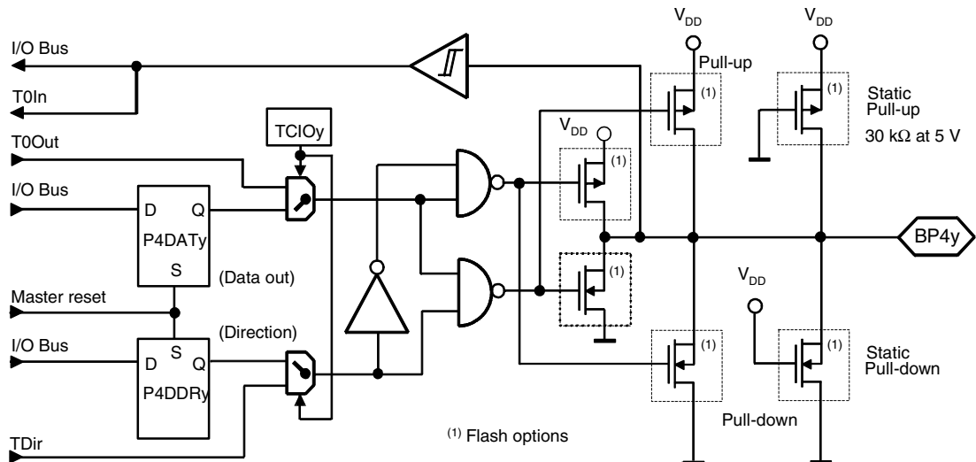
Figure 3-7. Bi-directional Port 4
