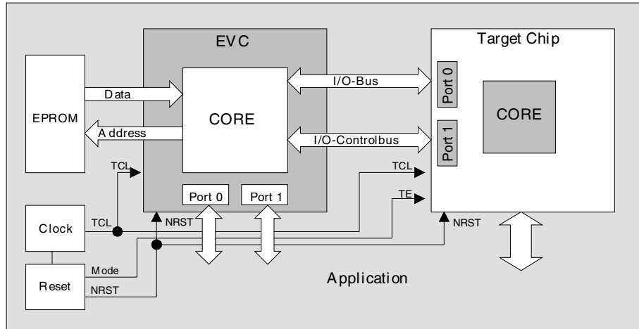
Figure 3-29. Emulation
