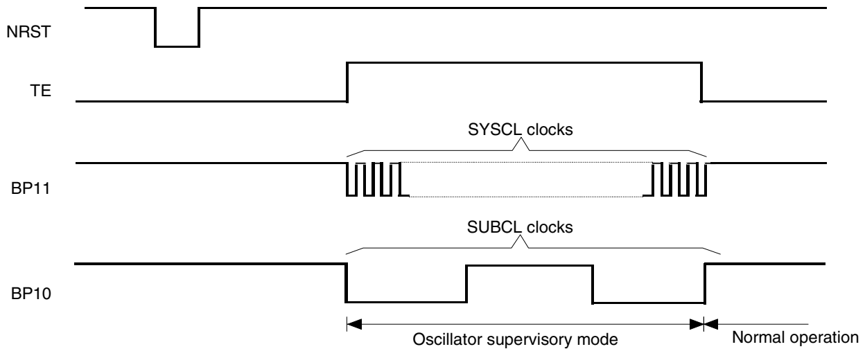
Figure 2-14. Clock Monitoring
