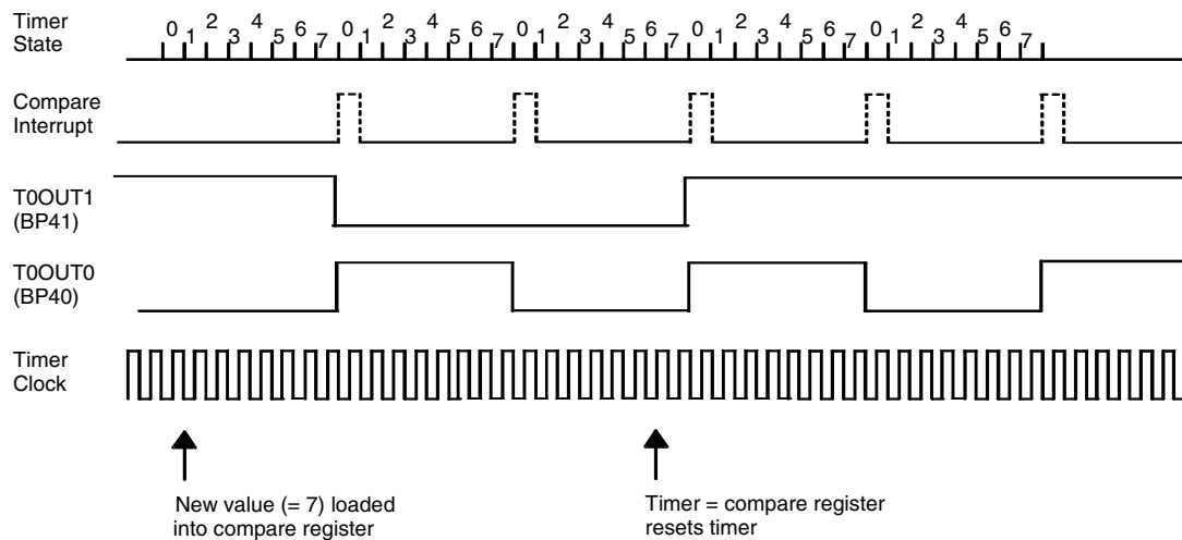
Figure 3-16. Modulated Melody Mode
