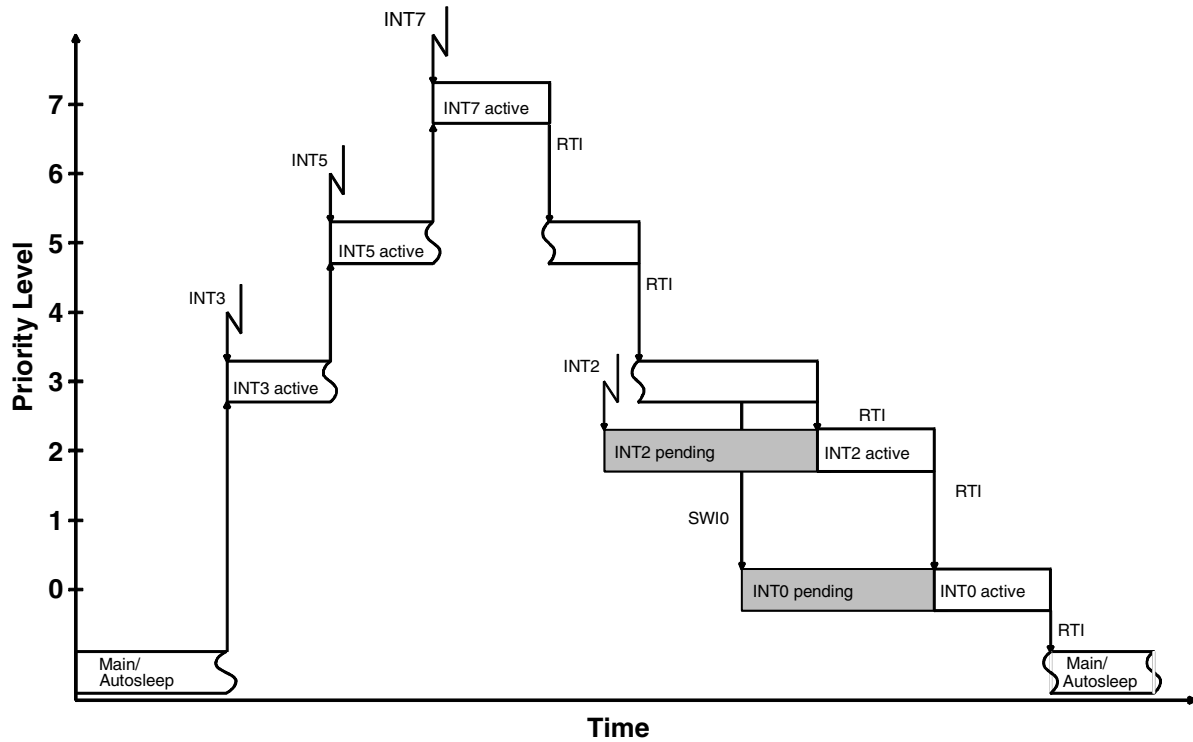
Figure 2-6. Interrupt Handling
