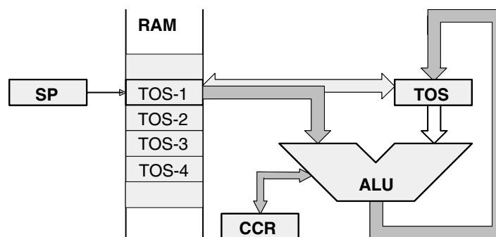
Figure 2-5. ALU Zero-address Operations
