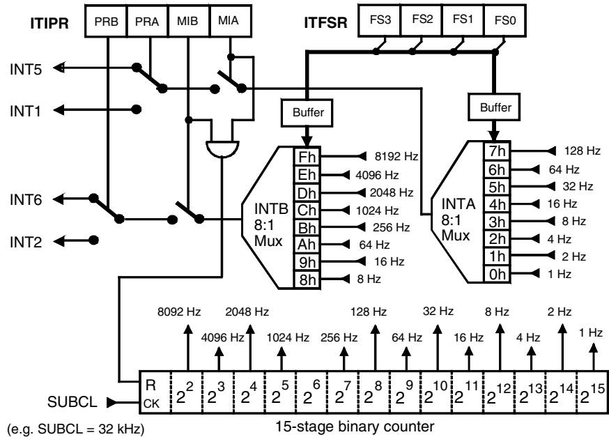
Figure 3-9. Interval Timers/Prescaler
