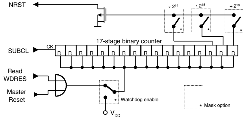
Figure 3-10. Watchdog Timer
