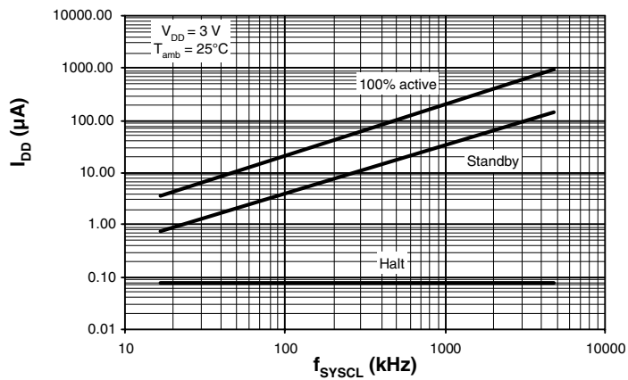
Figure 7-3. I_{\text{DD}} = f(f_{\text{SYSCL}}) , V_{\text{DD}} = 3 V
