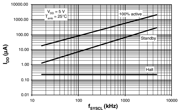
Figure 7-4. I_{\text{DD}} = f(f_{\text{SYSCL}}) , V_{\text{DD}} = 5 V
