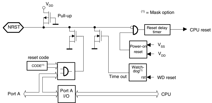
Figure 2-7. Reset Configuration
