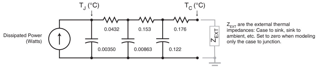
Figure 11, Transient Thermal Impedance Model
