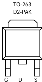
TO-263 D2-PAK Top View Drain Connected to Tab
