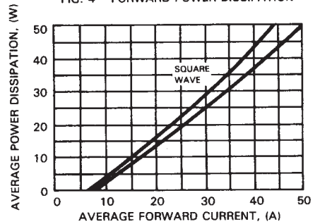
FIG. 4 - FORWARD POWER DISSIPATION
