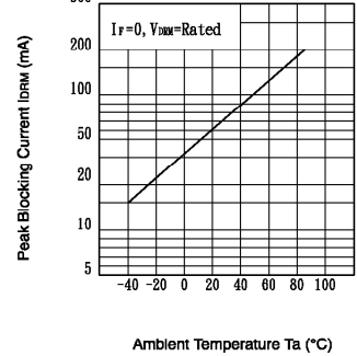
Fig.11 IDRM2, Leakage in Inhibit vs. Ambient Temperature
