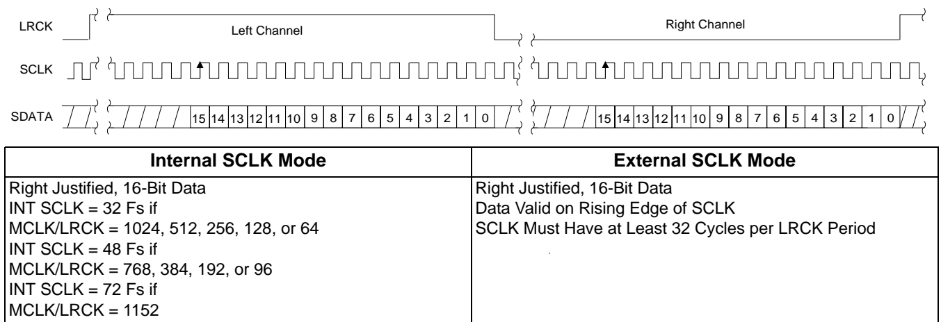
Figure 10. CS4348 Data Format (Right Justified 16)
