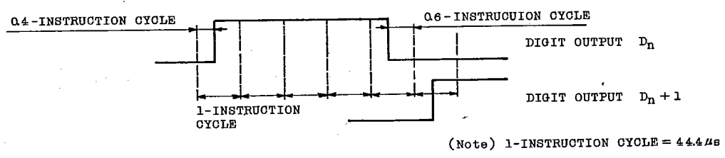
RELATION BETWEEN DIGIT OUTPUT SIGNAL TIMING AND INSTRUCTION CYCLE
