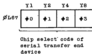
CORRESPONDING TABLE OF EXTERNAL DEVICE CHIP SELECT CODES
