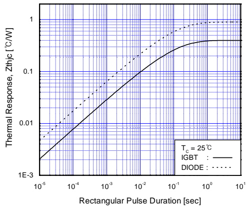
Fig 18. Transient Thermal Impedance
