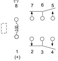
Terminal designations (Top view de-energized position)
