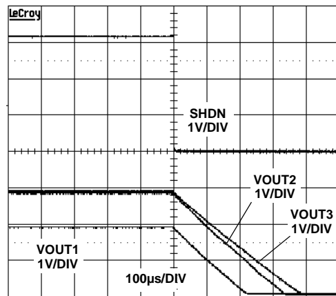
FIGURE 2. SHUTDOWN SEQUENCE
