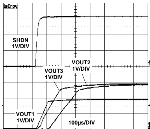
FIGURE 1. START-UP SEQUENCE
