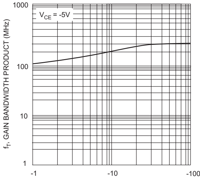
Fig. 7, Gain Bandwidth Product vs. Collector Current
