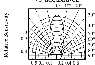
FIG.6 SENSITIVITY DIAGRAM
