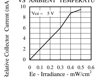
FIG.4 RELATIVE COLLECTOR CURRENT VS IRRADIANCE
