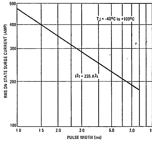
FIGURE 4 - SUB-CYCLE SURGES
