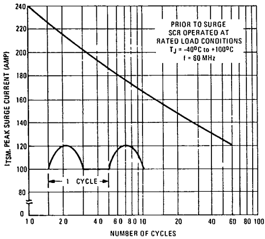
FIGURE 3 - 60 Hz SURGES
