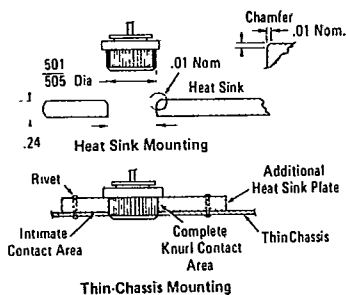
FIGURE 11 – MOUNTING DETAILS FOR PRESSFIT THYRISTORS
