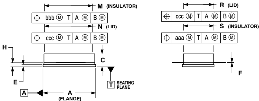
CASE 465C-02 ISSUE D NI-880S MRF6S19140HSR3
