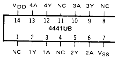
CONNECTION DIAGRAM (all packages)
