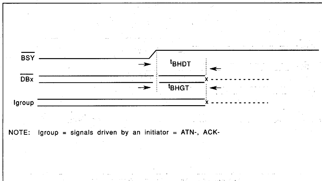
FIGURE 6-31. TIMING-INITIATOR TO BUS FREE
