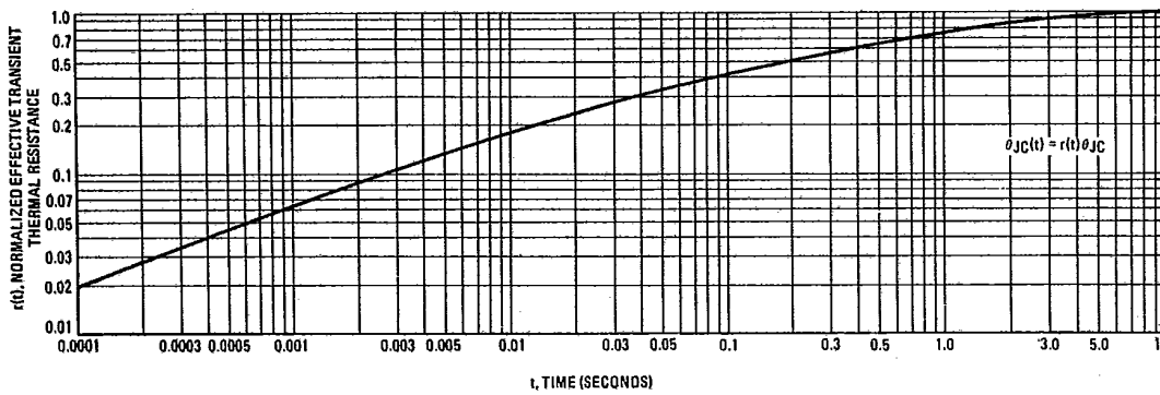
FIGURE 6 - THERMAL RESPONSE
