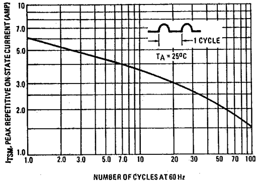
FIGURE 4 - SURGE RATINGS
