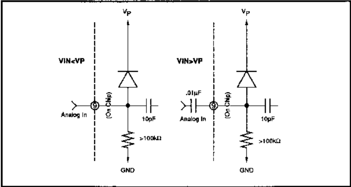
FIGURE 1: Input Coupling
