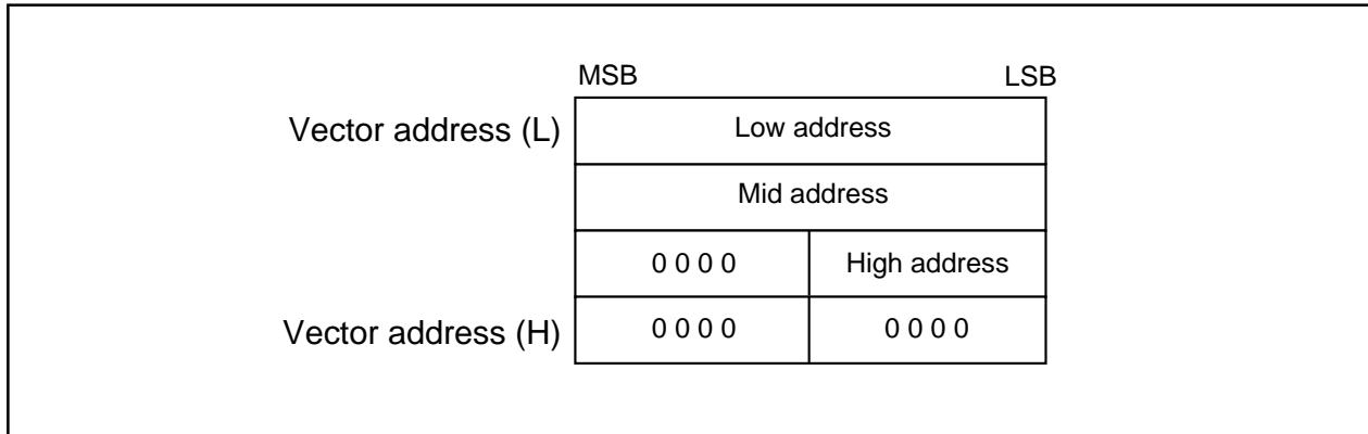
Figure 1.11.2. Interrupt Vector
